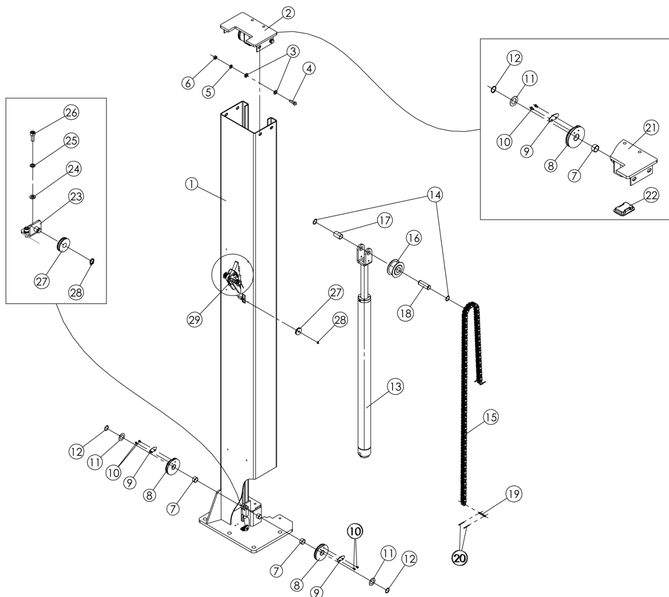
BN-2. 40ES-2 Column Assembling Explosion Drawing Lsit
